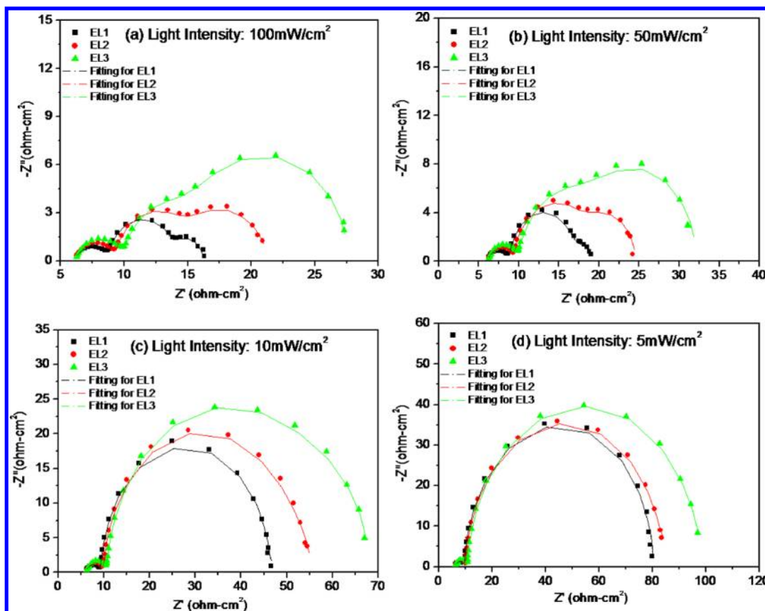
Figure 3. Nyquist plots and fitting curves of DSSCs with various electrolytes under various sun conditions: (a) 100, (b) 50, (c) 10, (d) 5 mW/cm 2 .
