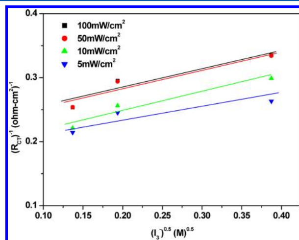
Figure 8. 1/R_{CT} as a function of the square root of [I_3^-] under various light intensities.
