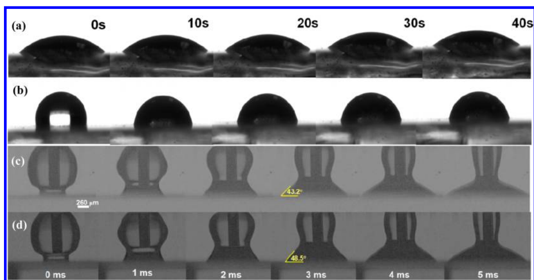
Figure 8. Dynamic process for DI water droplet permeation through (a) as-prepared NG3 film and (b) aged NG3 film (1000 cycles). Snapshots of cobalt electrolyte droplet permeation through (c) as-prepared NG3 film and (d) aged NG3 film (1000 cycles).
