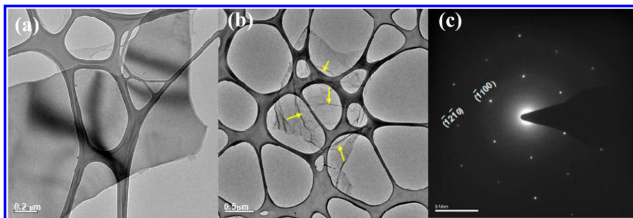
Figure 2. TEM images of (a) flaky graphene nanosheet and (b) curved NG; the yellow arrows show the obvious wrinkle. (c) The corresponding SAED.
